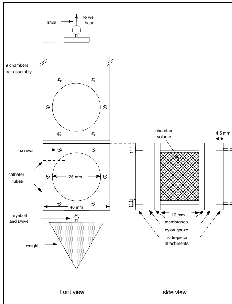
Figure 3. Diffusion Chambers Used in In Situ Pathogen Inactivation Studies (in front and side view, from Pavelic et al , 1998a)
